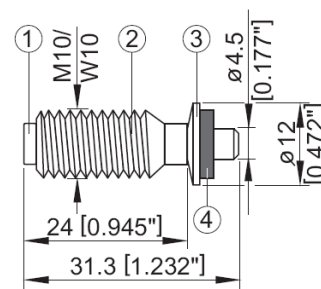
X-BT W10-24-6 SN12-R X-BT M10-24-6 SN12-R
