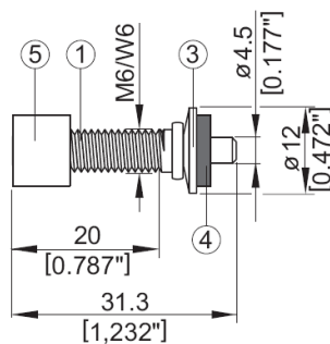
X-BT W6-24-6 SN12-R X-BT M6-24-6 SN12-R
